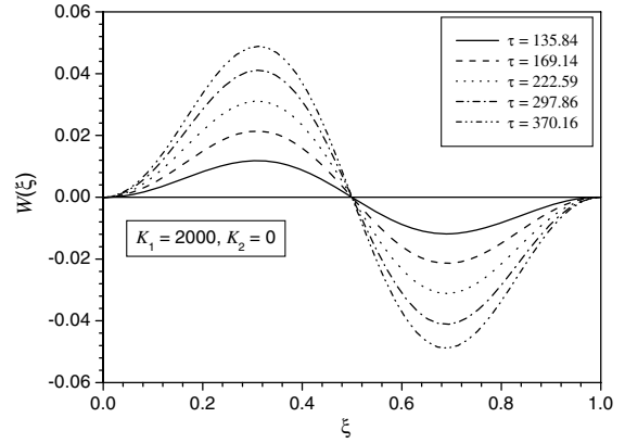
b) K_1 = 2000
