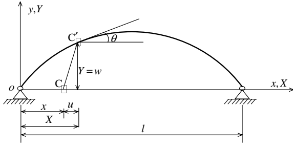
Fig. 2 A buckled configuration of a pinned-pinned beam.
